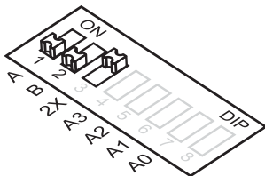
Termination OFF
