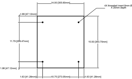
Top/Bottom View
